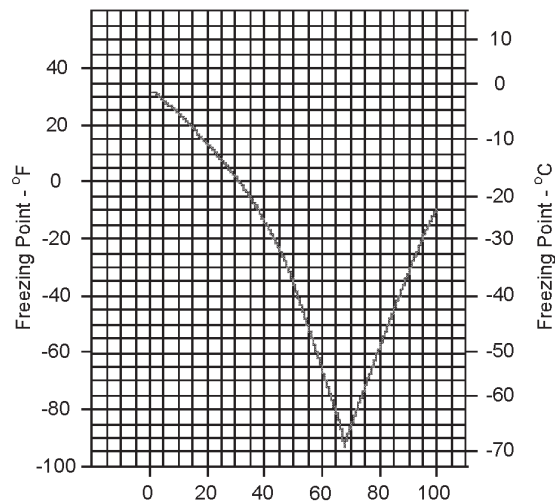
Ethylene Glycol Antifreeze Percent by Volume
