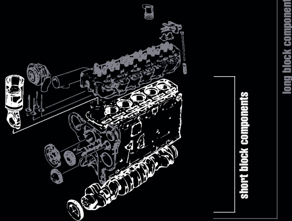
3406 Engine
