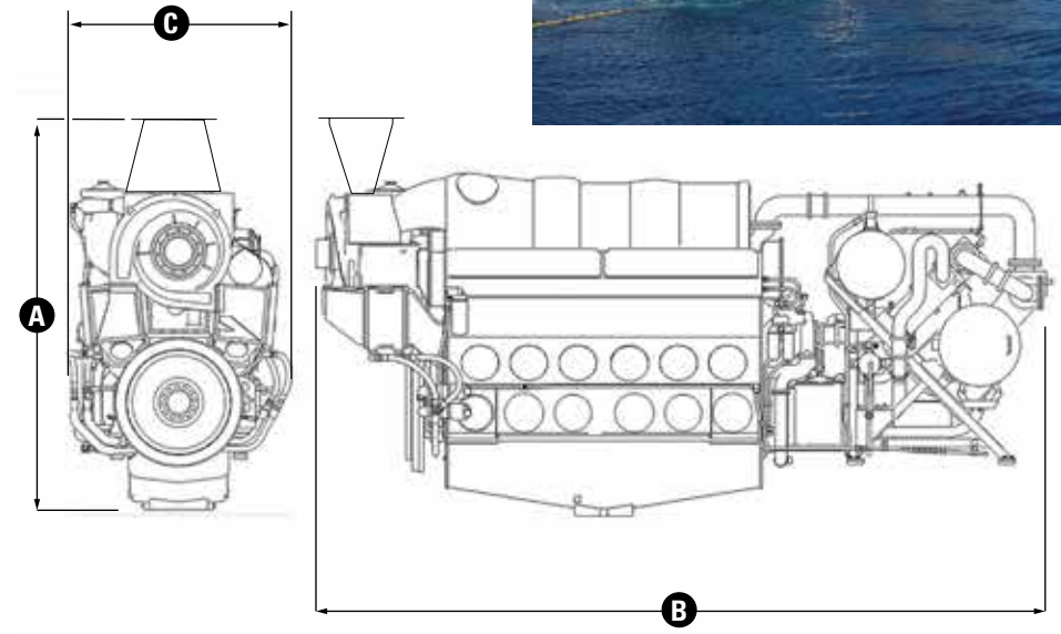
E 23 ENGINE
